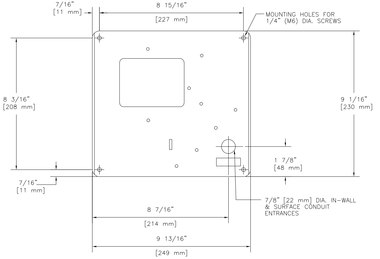
FIGURE 6 - GX HAND DRYER
