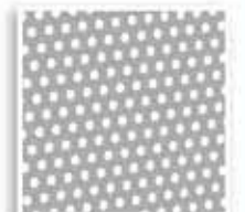
30% Open Area Staggered Pattern 1/8" Diameter 7/32" Spacing
