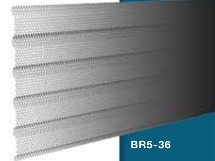
10% Open Area Reverse Pattern 1/8" Diameter 3/8" Spacing
