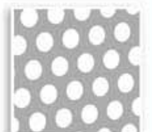
40% Open Area Staggered Pattern 3/8" Diameter 9/16" Spacing
