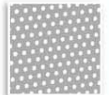
23% Open Area Staggered Pattern 1/8" Diameter 1/4" Spacing
