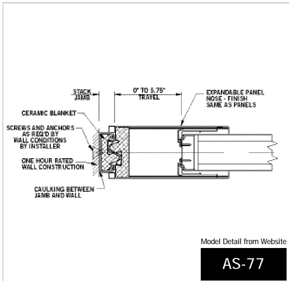
Expandable Panel w/ Jamb
