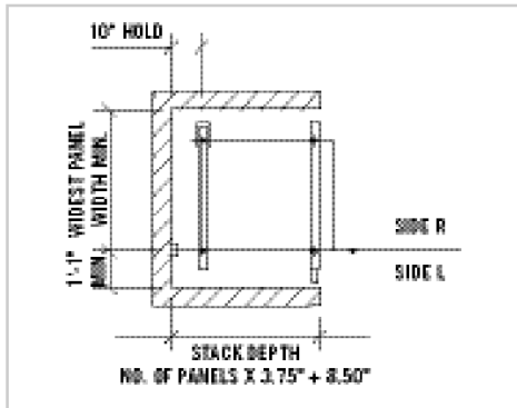
Remote Expandable Closure - Offset Stack Right Angle
