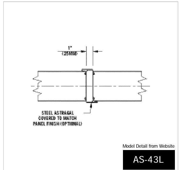
Hinged Panel Meeting w/ Pass Door Astragal
