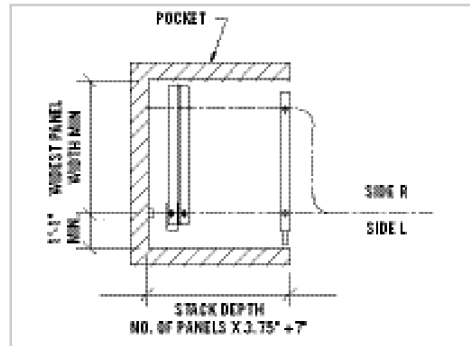
Bi-fold Expandable Closure - (Flat Stack) Smart Track
