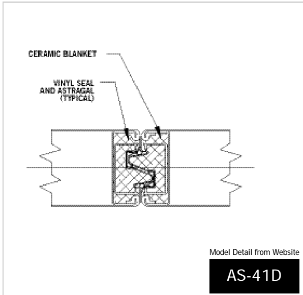
Standard Panel Joint
