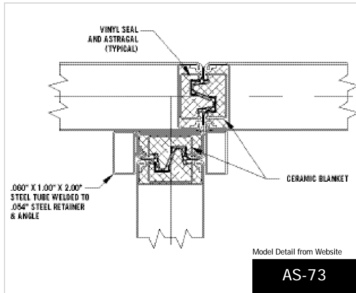
Intersecting Wall
