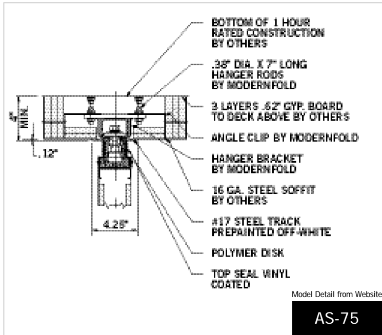
#17 Track System Bracket Mount (Right Angle Shown)
