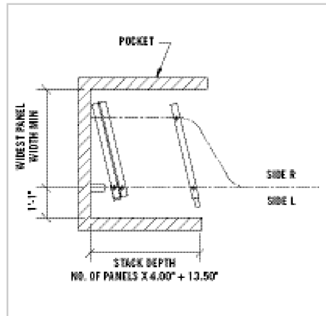
Bi-fold Expandable Closure - (Angle Stack) Smart Track
