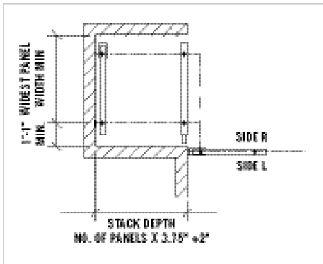
Remote Expandable Closure - Parallel Stack (Angle Stack) Smart Track
