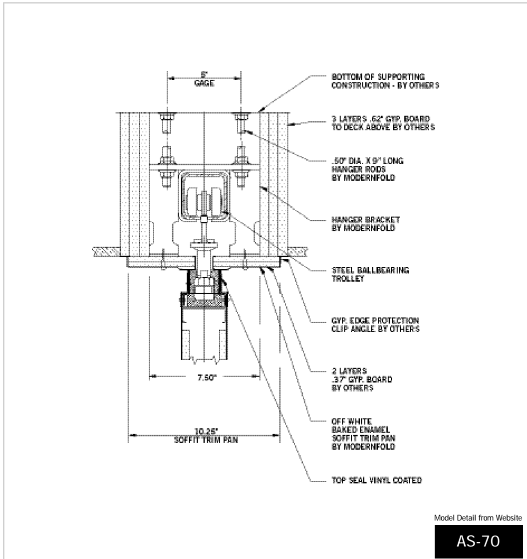
#14 Track System Bracket Mount (Smart Track Shown)
