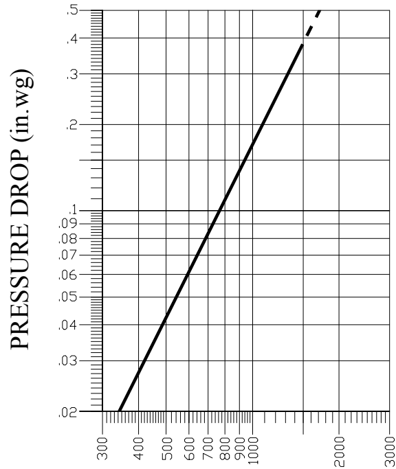
AIR VELOCITY IN FEET PER MINUTE THROUGH FREE AREA LOUVER SIZE = 48" X 48"
