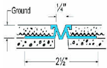
Vinyl Control Joint
