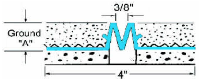
scale varies with dimension "M" Type Expansion Joint
