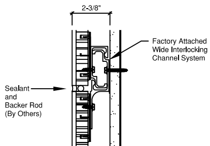
2A Wide Interlocking Channel System
