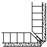
Quirk Miter Corner
