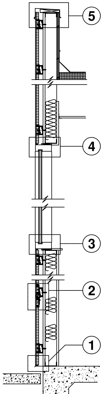
Wall Section
