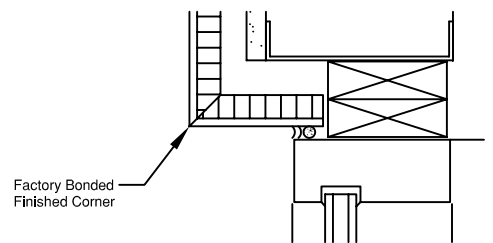
4B Window Head - Recessed
