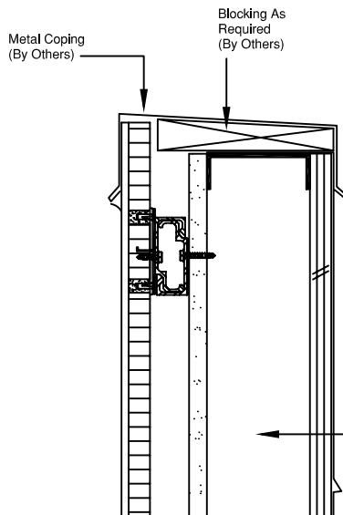
5A Metal Coping Detail
