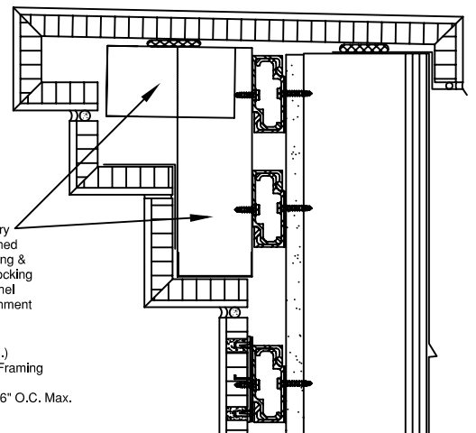
5B Stone Panel Cornice
