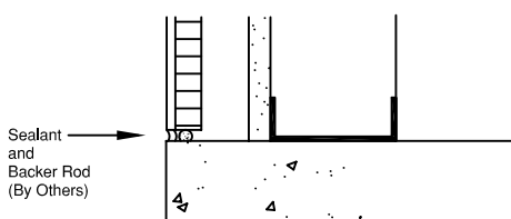
1A Base Detail
