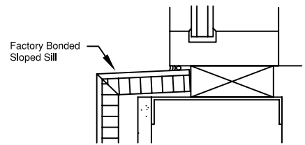
3B Window Sill - Recessed
