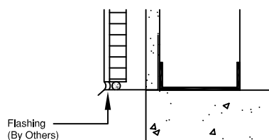
1B Base Detail
