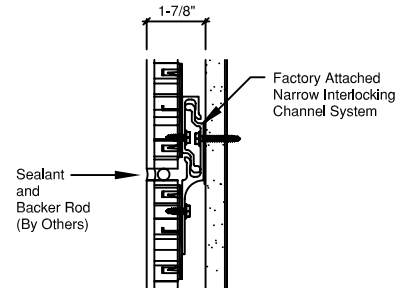
2B Narrow Interlocking Channel System
