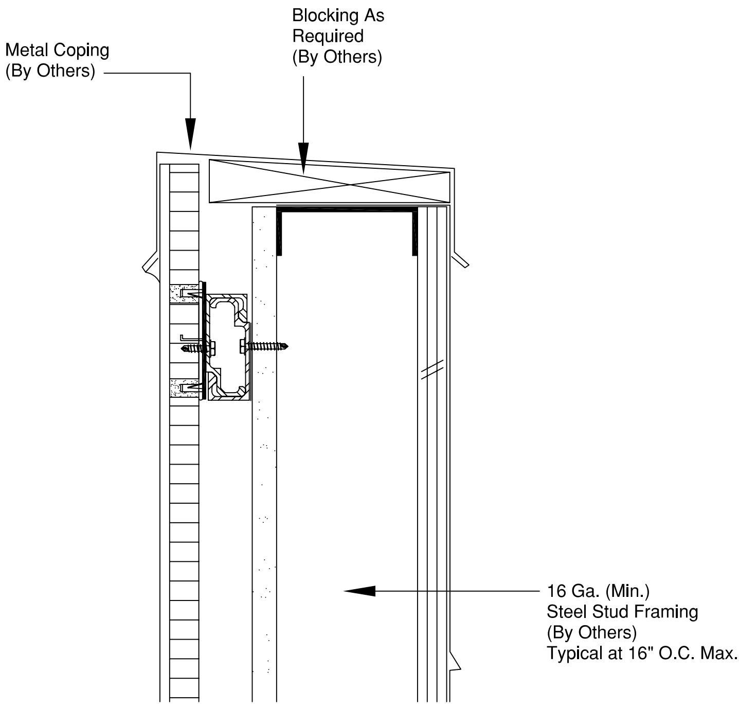
5A Metal Coping Detail
