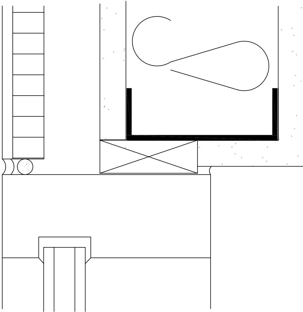
4A Window Head - Flush
